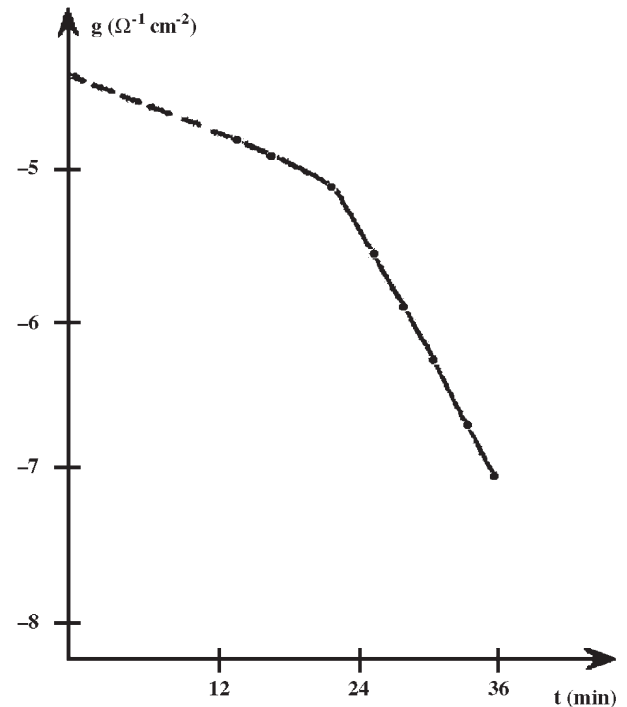
Fig. 6. Kinetics of the conductance decrease after removal from the one membrane side of metamphocin added to its two sides at the initial concentration of 2 \times 10^{-7} M. The applied potential was 100 mV. Aqueous solution: pH 6.5, 2 M KCl, temperature 24 °C. Membrane composition: 2:1 molar ratio of phospholipid:cholesterol.
